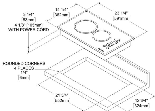
COUNTERTOP CUTOUT DIMENSIONS 2-BURNER LARGE LANDSCAPE
