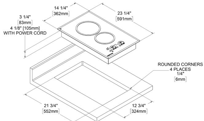
COUNTERTOP CUTOUT DIMENSIONS 2-BURNER LARGE PORTRAIT
